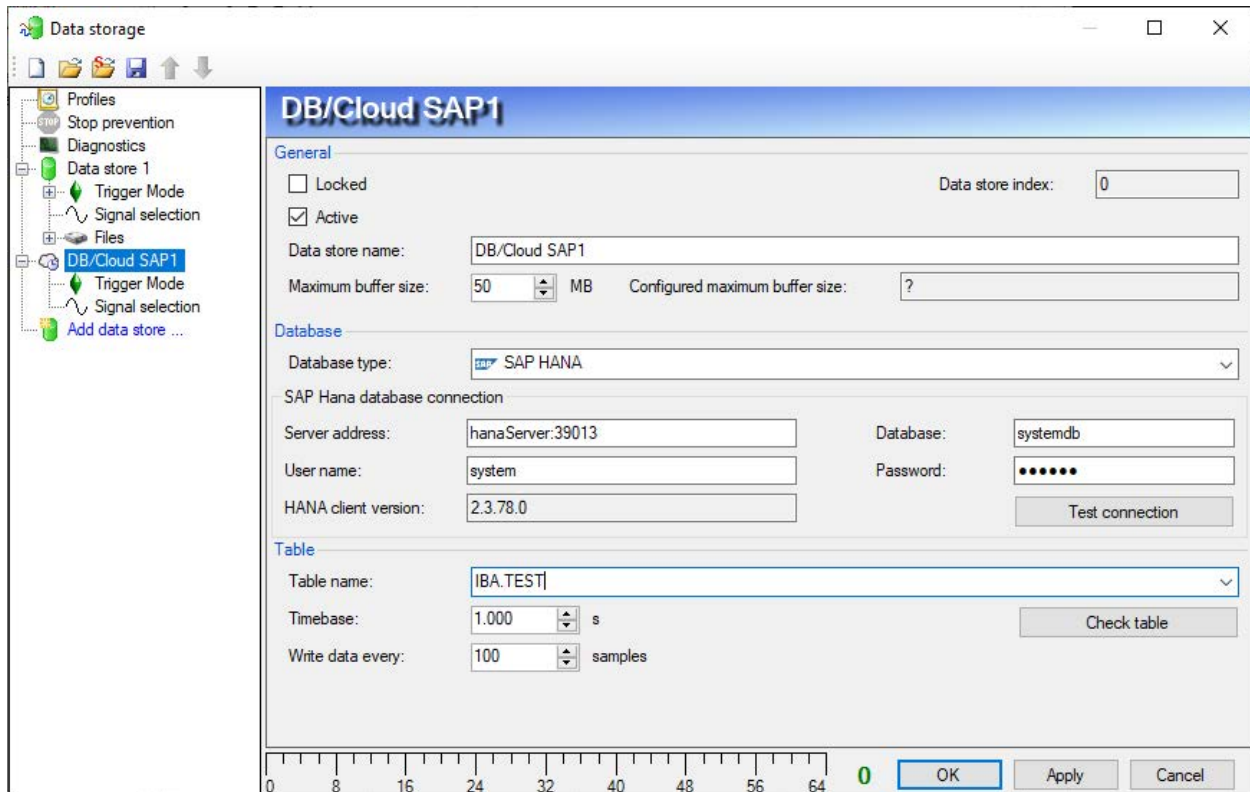
Fig. 2: Configuring DB/Cloud data store
