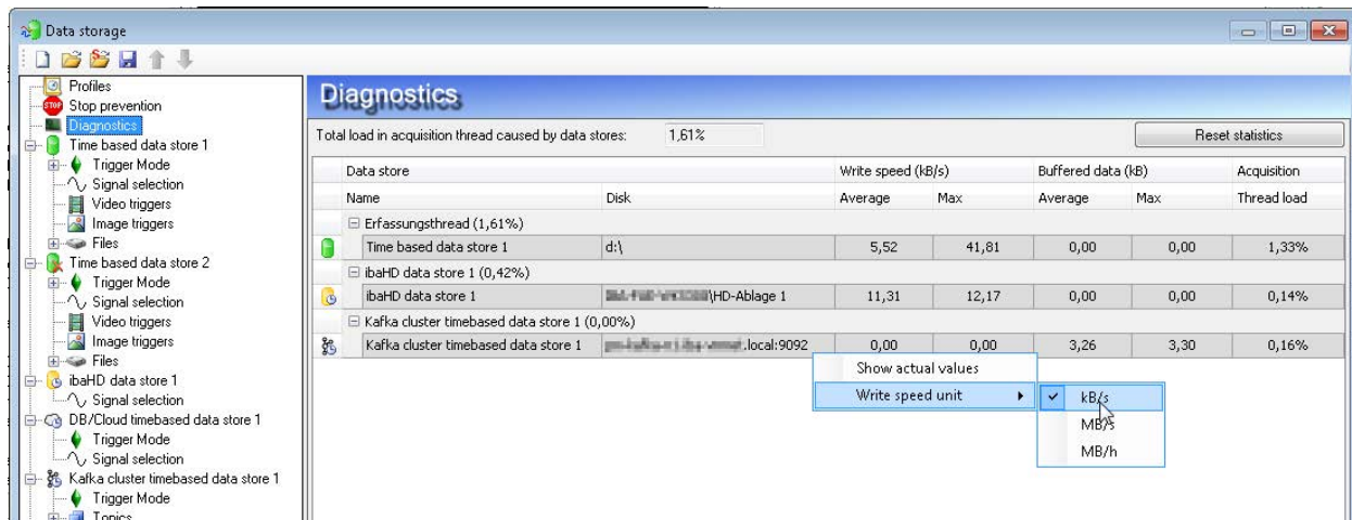
Fig. 12: Diagnostics of data stores
